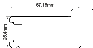
57mm Chamfer D-Mould Stile
