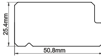
50mm Chamfer Rebate Stile
