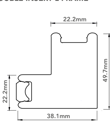
Double Insert L Frame 50mm
