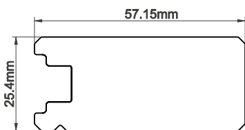
57mm Chamfer Butt Stile
