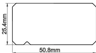
50mm Chamfer Butt Stile
