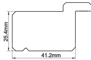
41.3mm Chamfer D-Mould Stile
