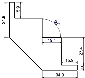
(Deco Frame) 32mm
