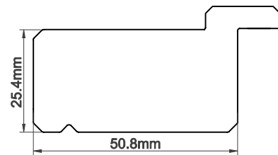
50mm Chamfer D-Mould Stile
