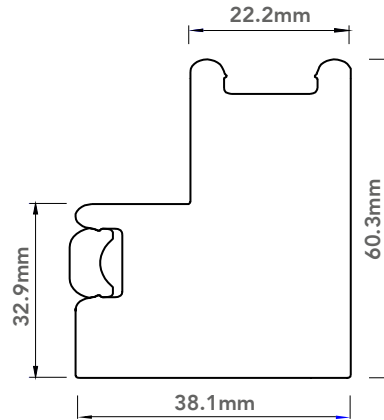
Double Insert L Frame 60mm
