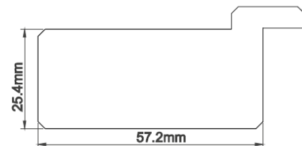
57.2mm Flat D-Mould Stile
