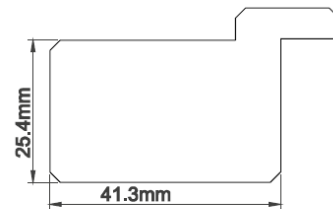
41.3mm Flat D-Mould Stile
