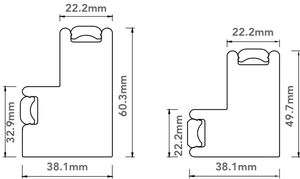
Double Insert L Frame 50mm
