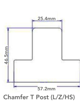
Chamfer T Post (L/Z/HS)
