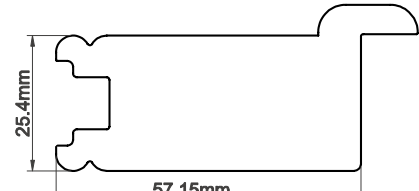
57mm D-Mould Stile
