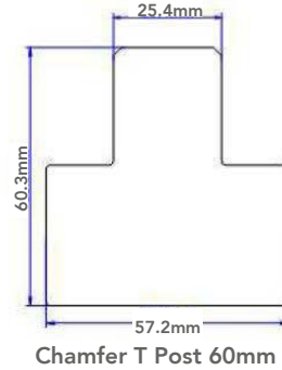
Chamfer T Post 60mm
